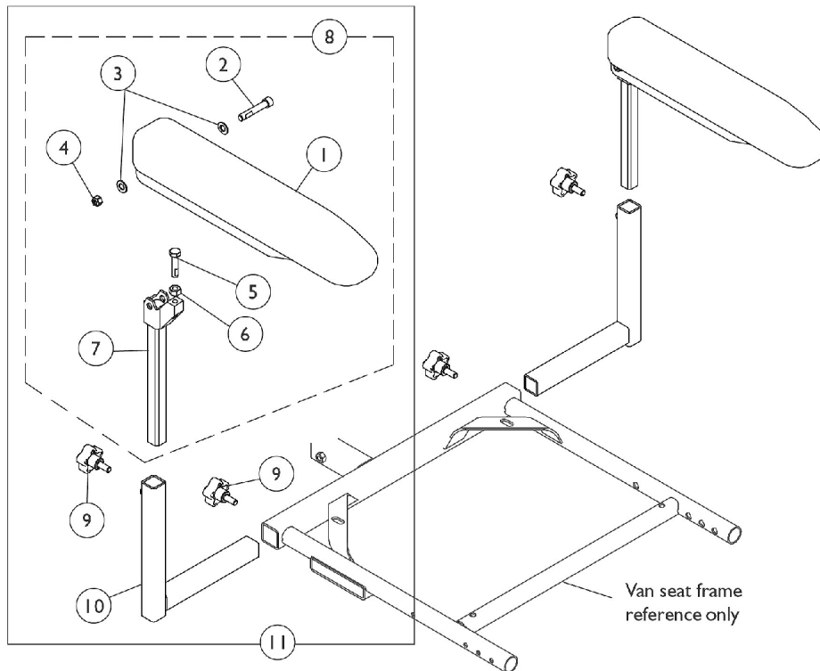
Adjustable Height / Width Arm Assembly
