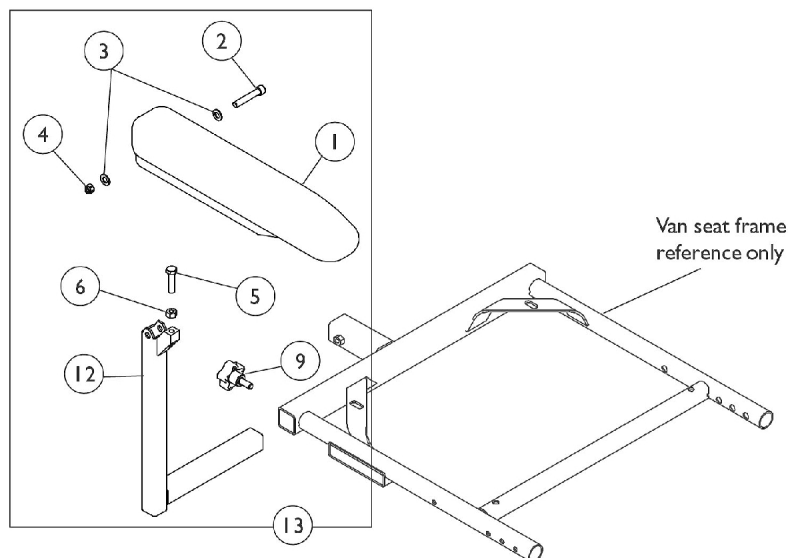
Fixed Height / Adj. Width Arm Assembly
